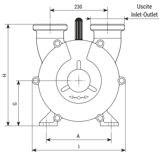
NAUTIC 80 Inox F
