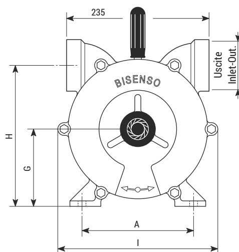
NAUTIC 70 F NAUTIC 70 Inox F
